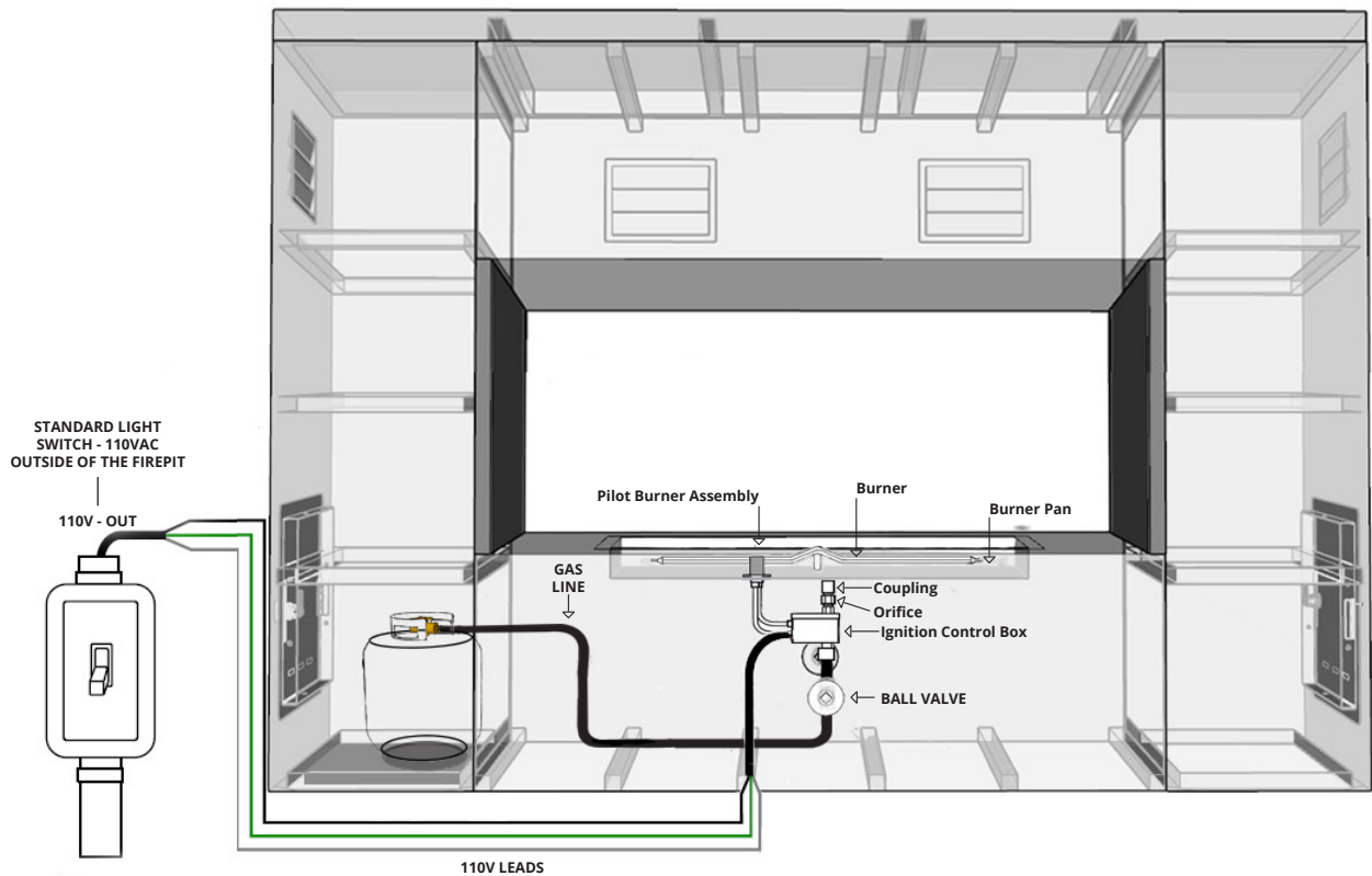
Figure 3.4 | Using a standard light switch
