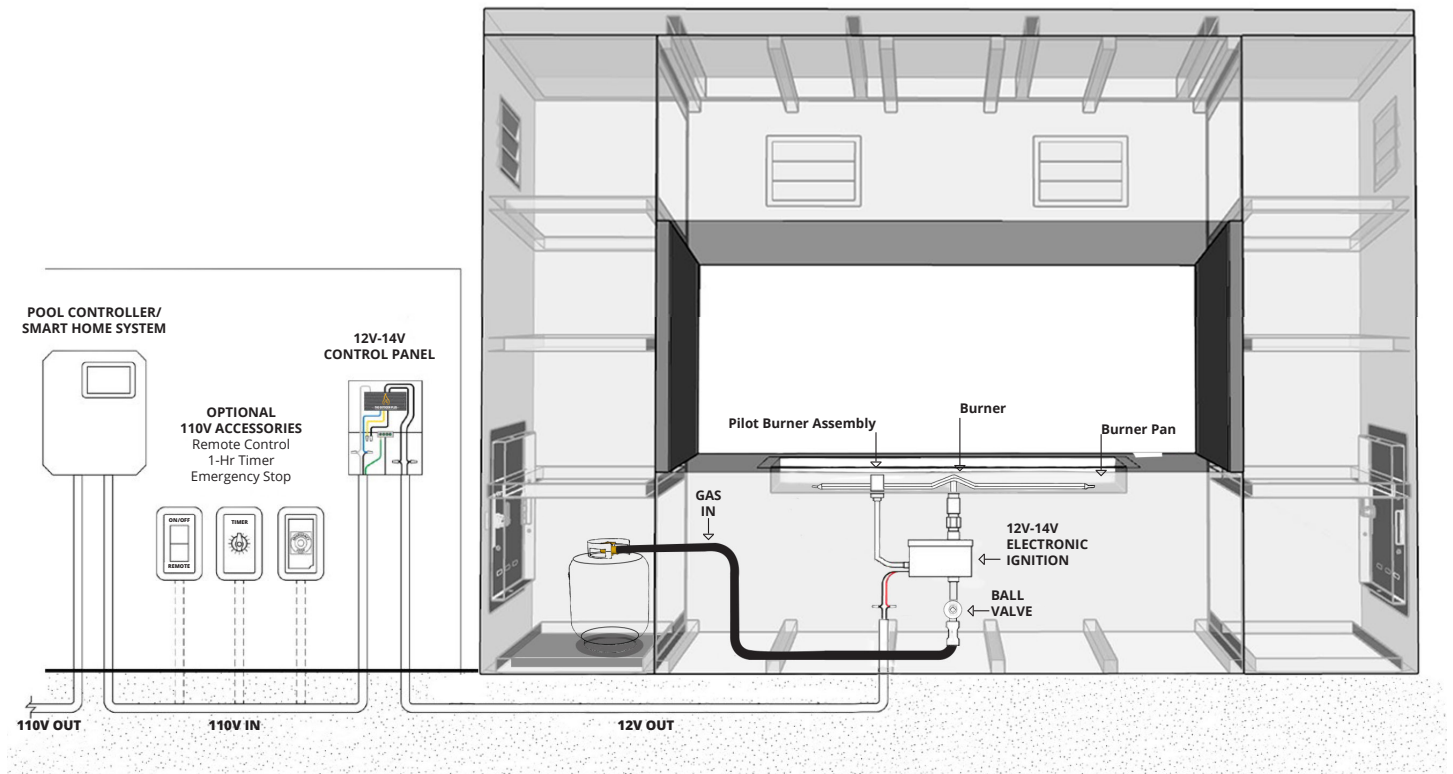
Figure 2.2 | Using an Automated Pool Controller with a Low Voltage Control Panel
