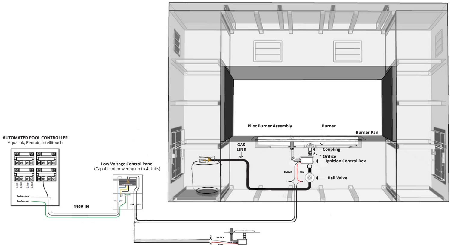
Figure 2.2 | Using an Automated Pool Controller with a Low Voltage Control Panel
