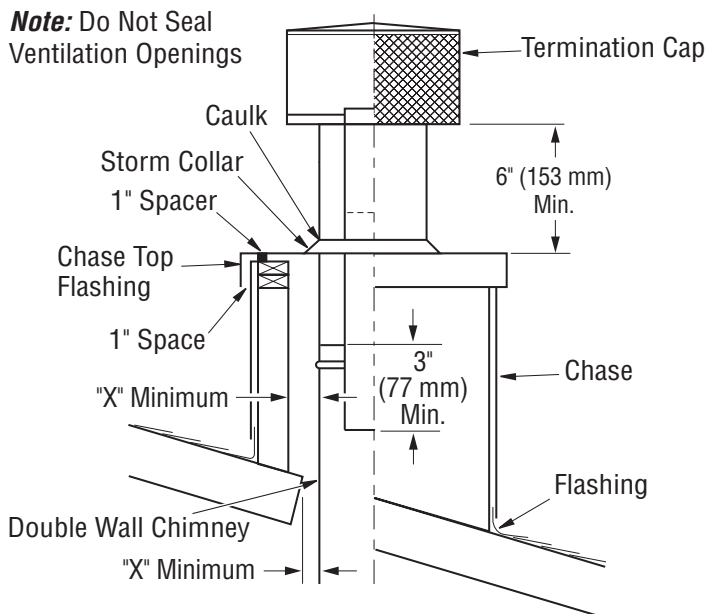
Figure 29 - Chase Installation
