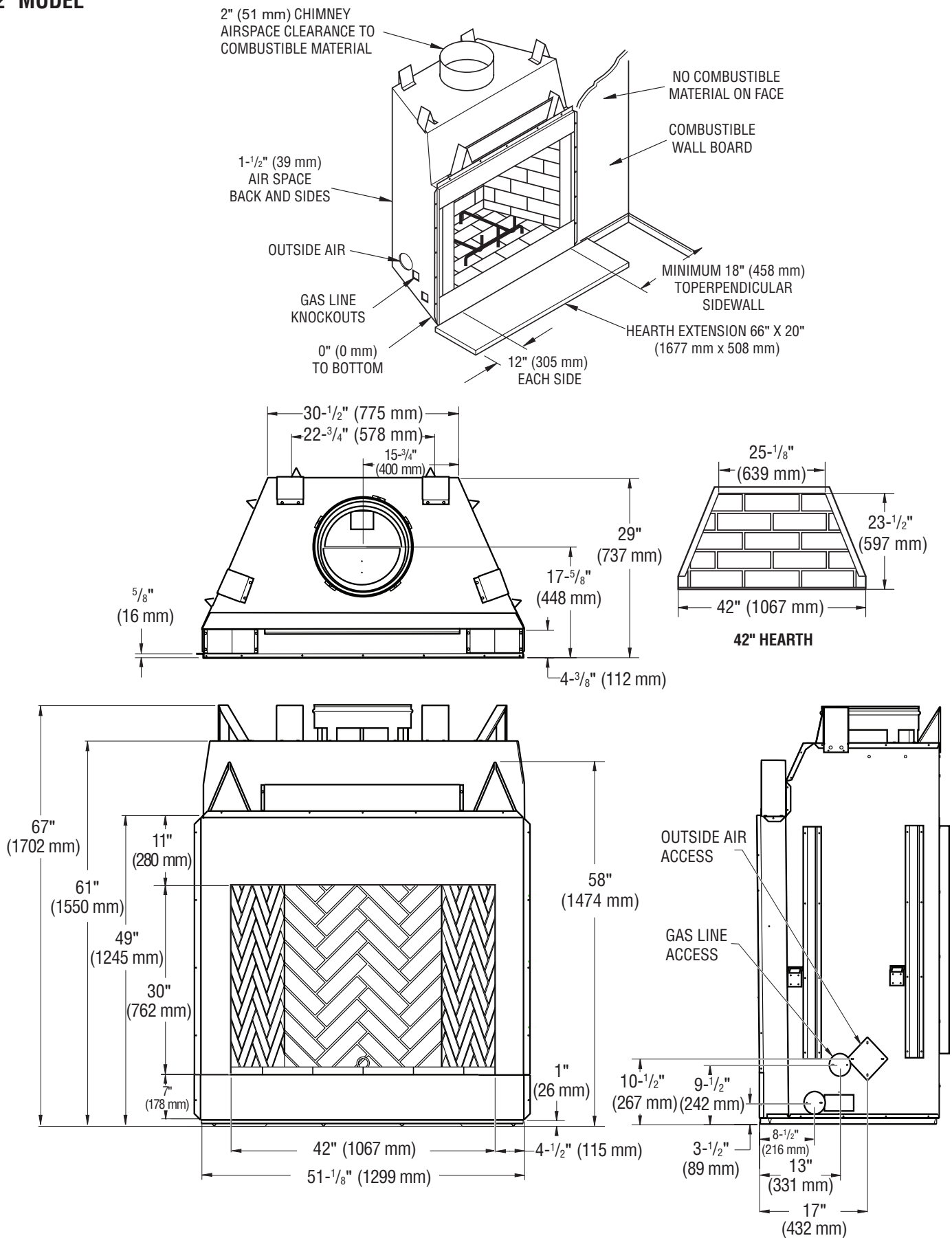
Figure 2 - 42" Models
