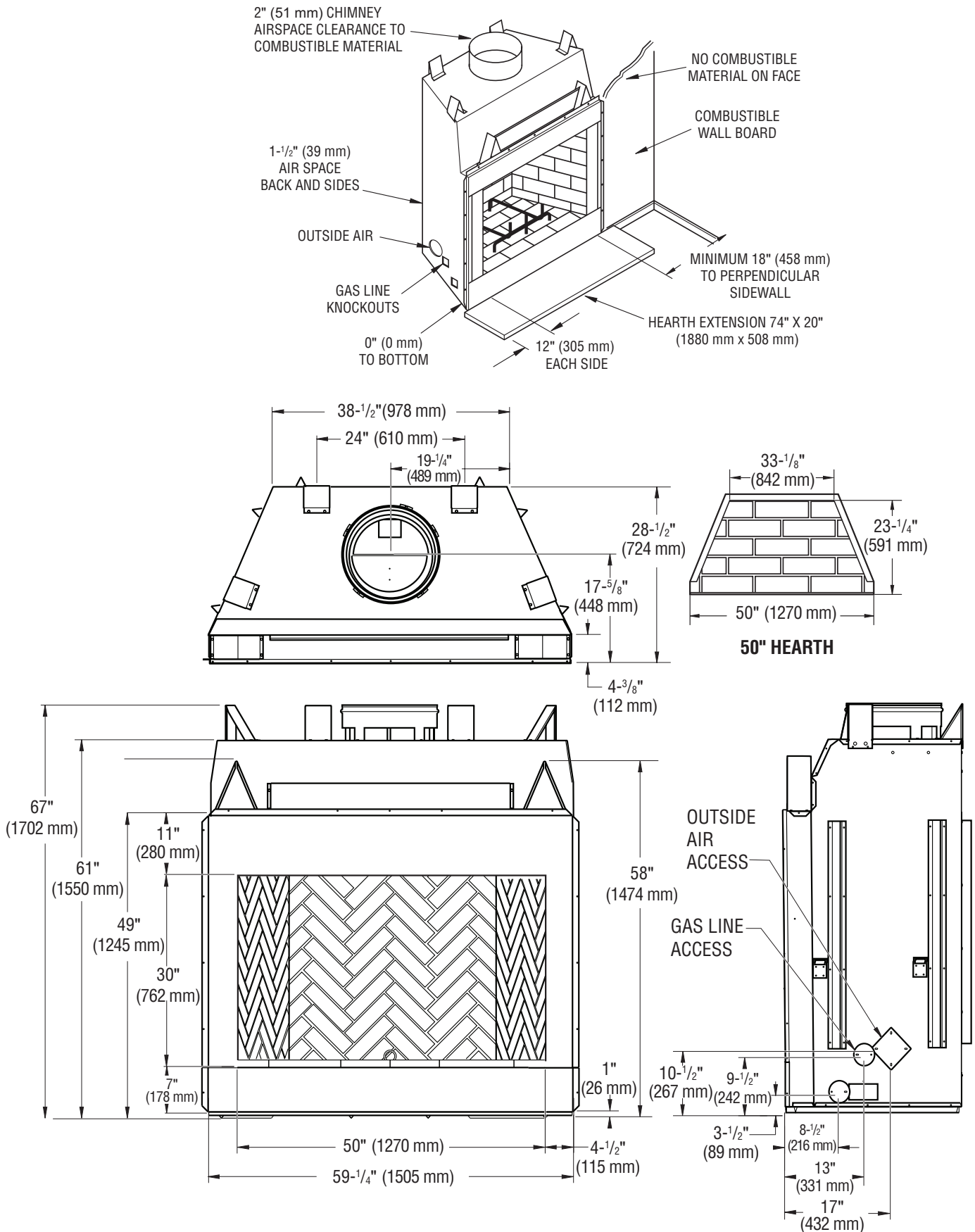
Figure 3 - 50" Models
