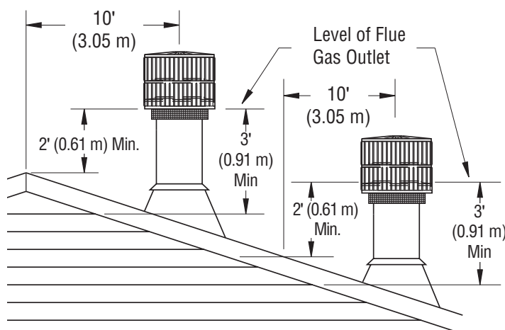
Figure 20 - 10 Foot Rule
