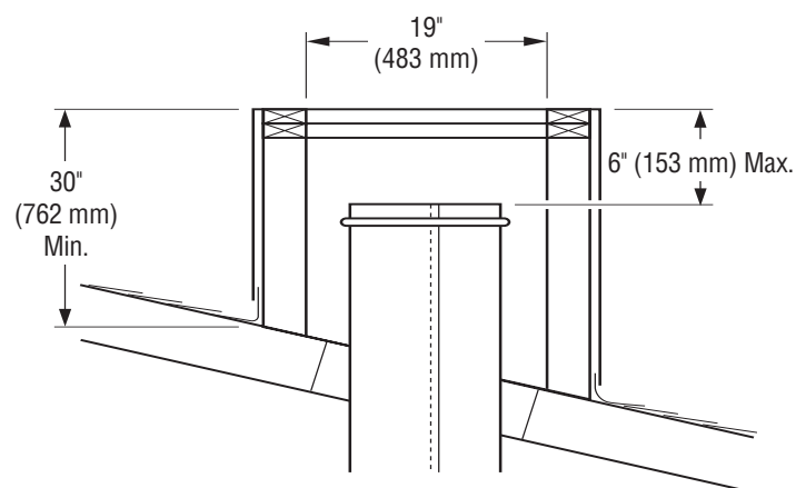
Figure 21 - Constructing Chase
