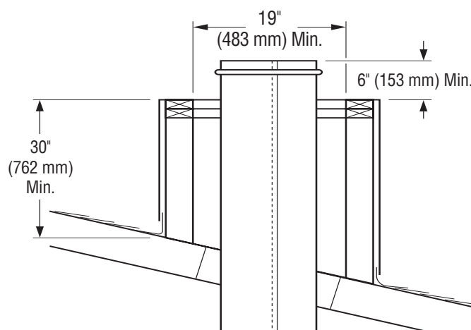
Figure 25 - Constructing Chase
