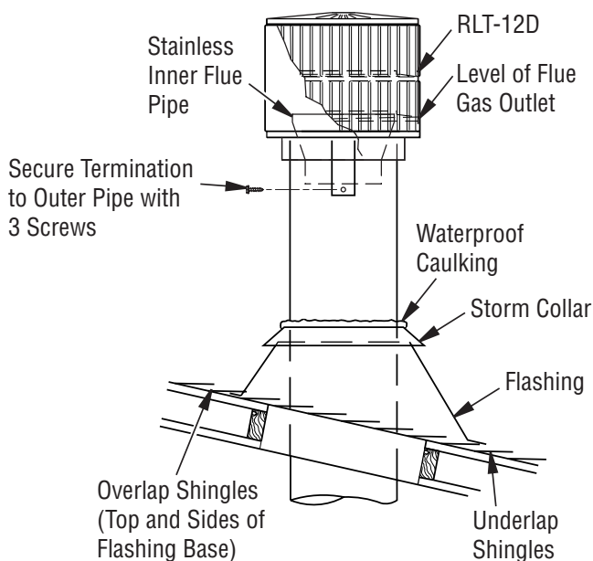
Figure 18 - Termination
